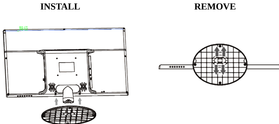
Figure.1. Installing and Removing the Base
