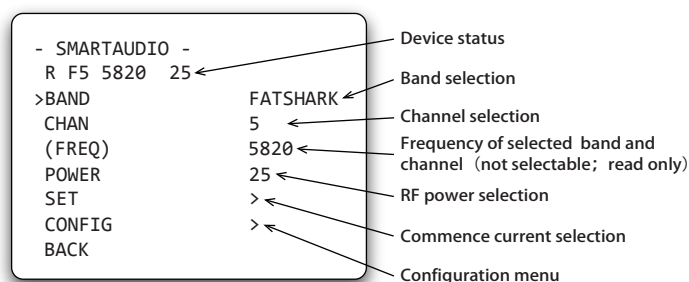
SmartAudio VTX top menu (Band/Channel mode)
