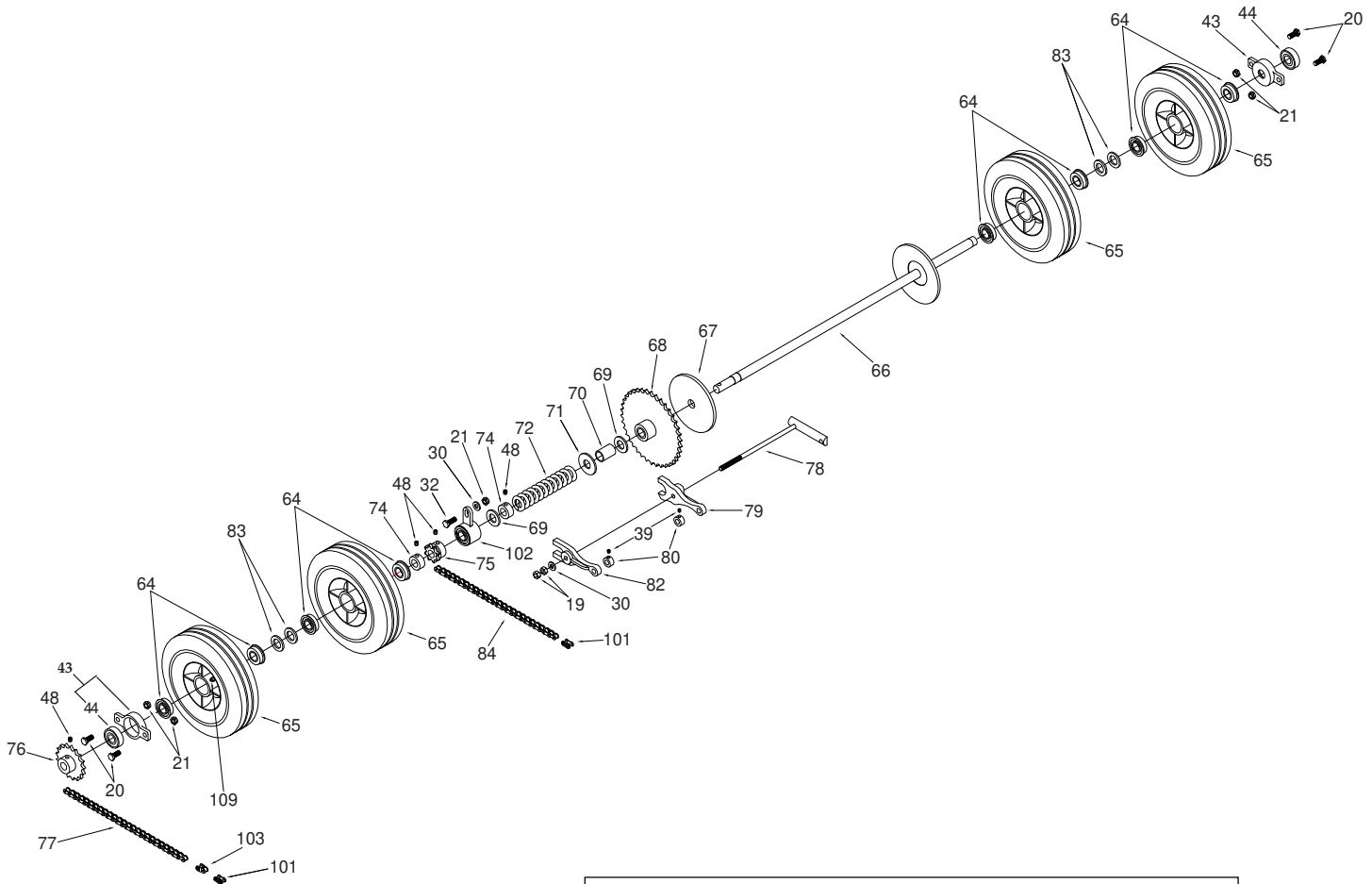
25301-A 25" Drive Shaft Assembly
