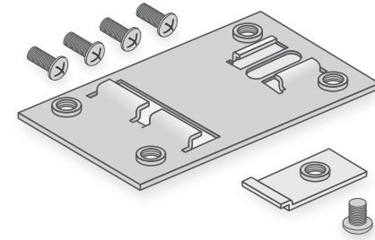
Metal bracket with T-bar and lock screw for ceiling mounting and 4 short screws to attach the plastic mount to the metal bracket
