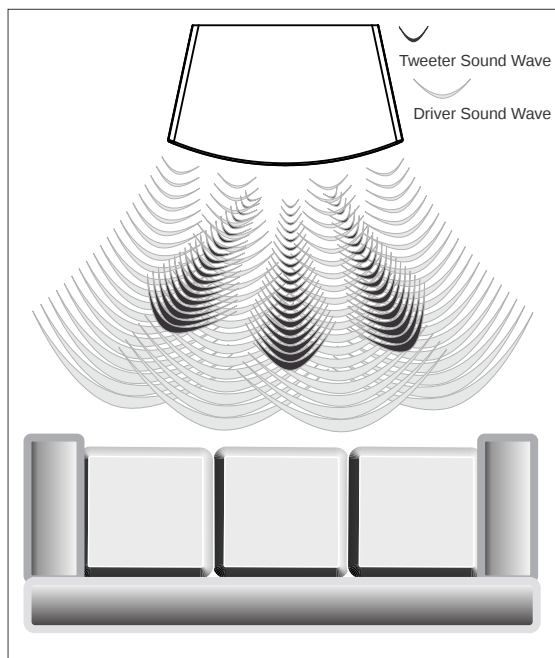
Figure 1. Theia's Acoustic Array System Design (AASD) audio dispersion.
