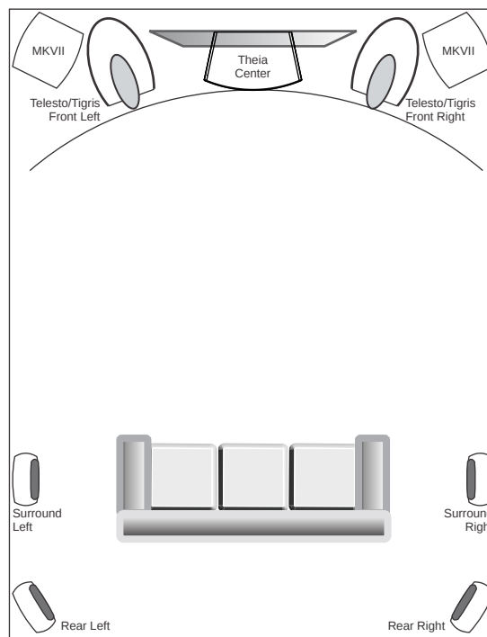
Figure 8. Typical speaker placement in 7.1 Theater System
