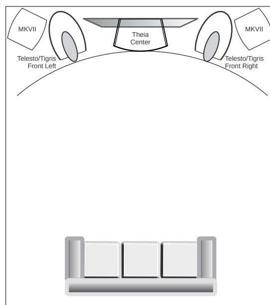
Figure 5. Typical speaker & subwoofer placement in 3.1/2 theater system
